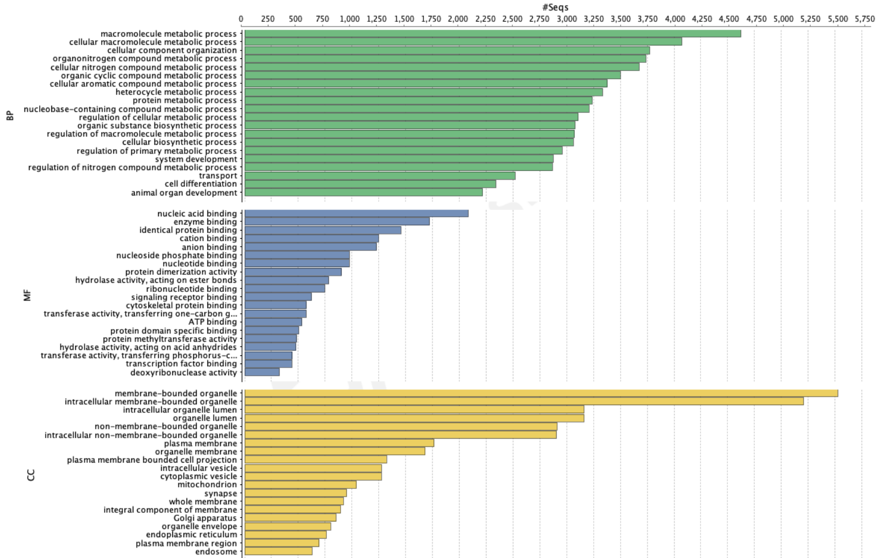
Figure S2. Level four GO terms for the SPAdes assembly with kmer 31.
