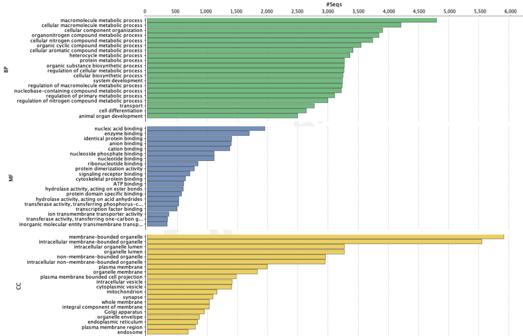
Figure S1. Level four GO terms for the Trinity assembly with kmer 32.
