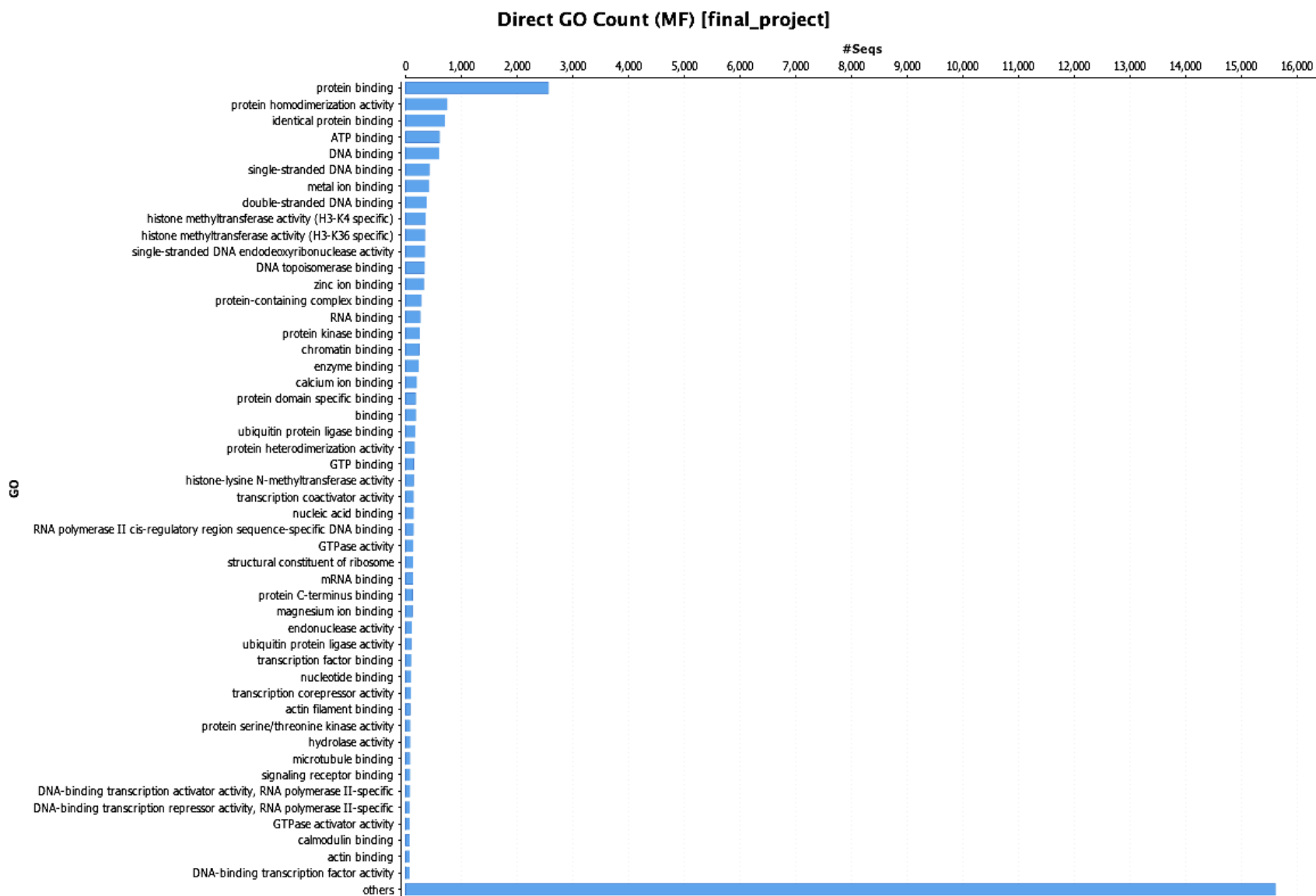
Figure S5. Top GO functions associated to the annotated proteins in the non-redundant merged transcriptome.
