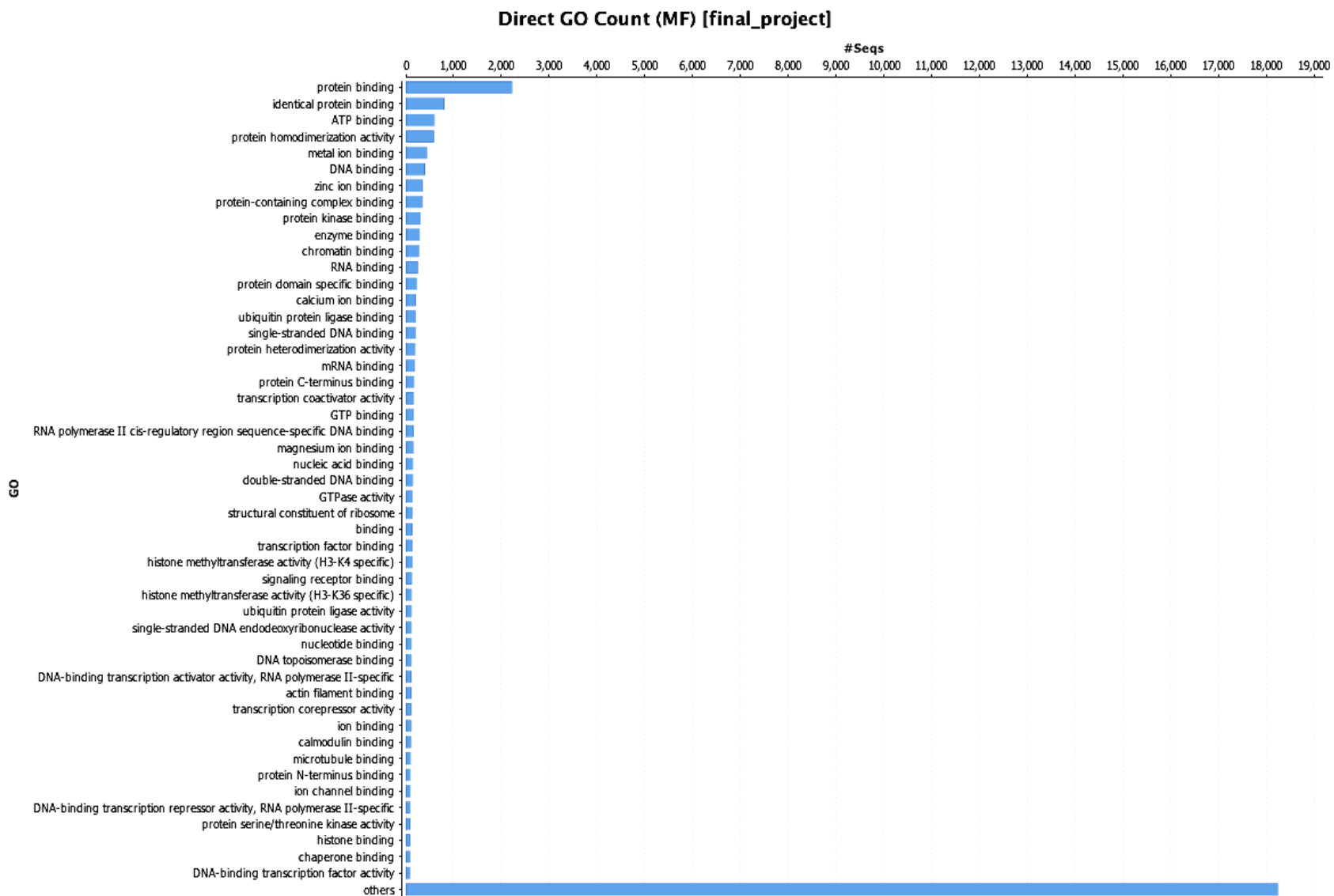
Figure S6. Top GO functions associated to the annotated proteins in the Trinity kmer 32 transcriptome
