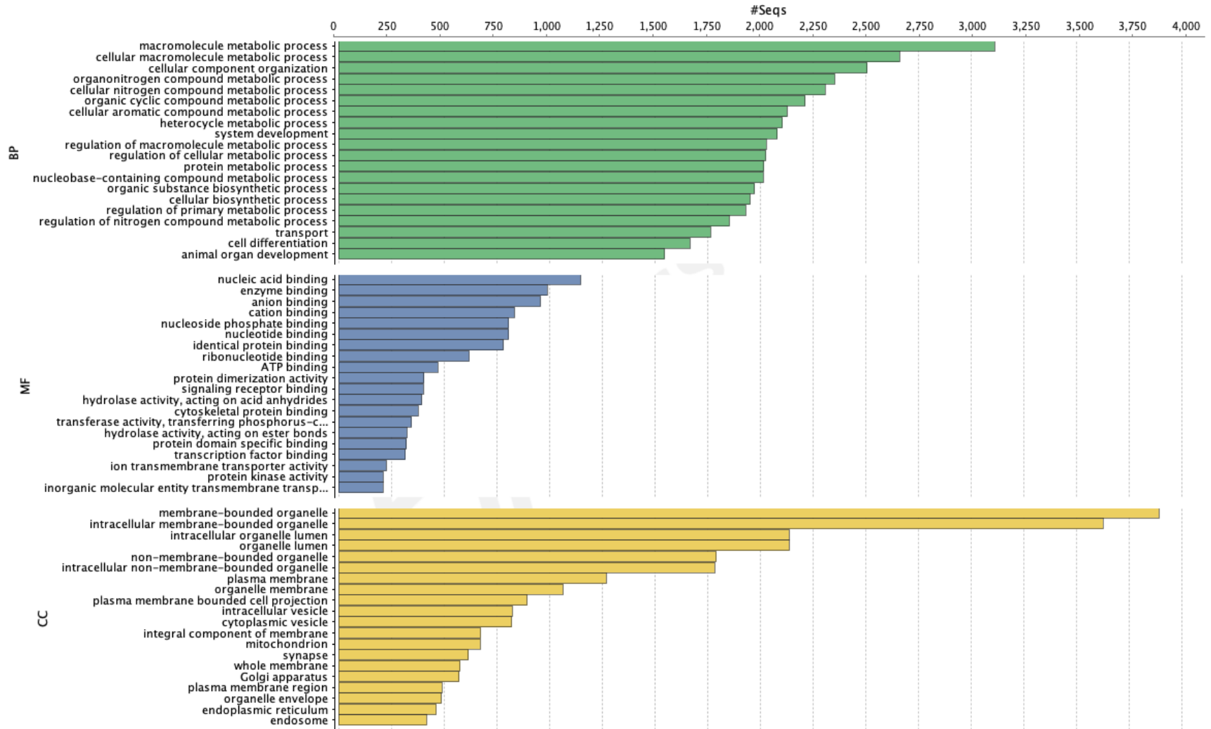
Figure S3. Level four GO terms for the Soapdenovo assembly with kmer 63..
