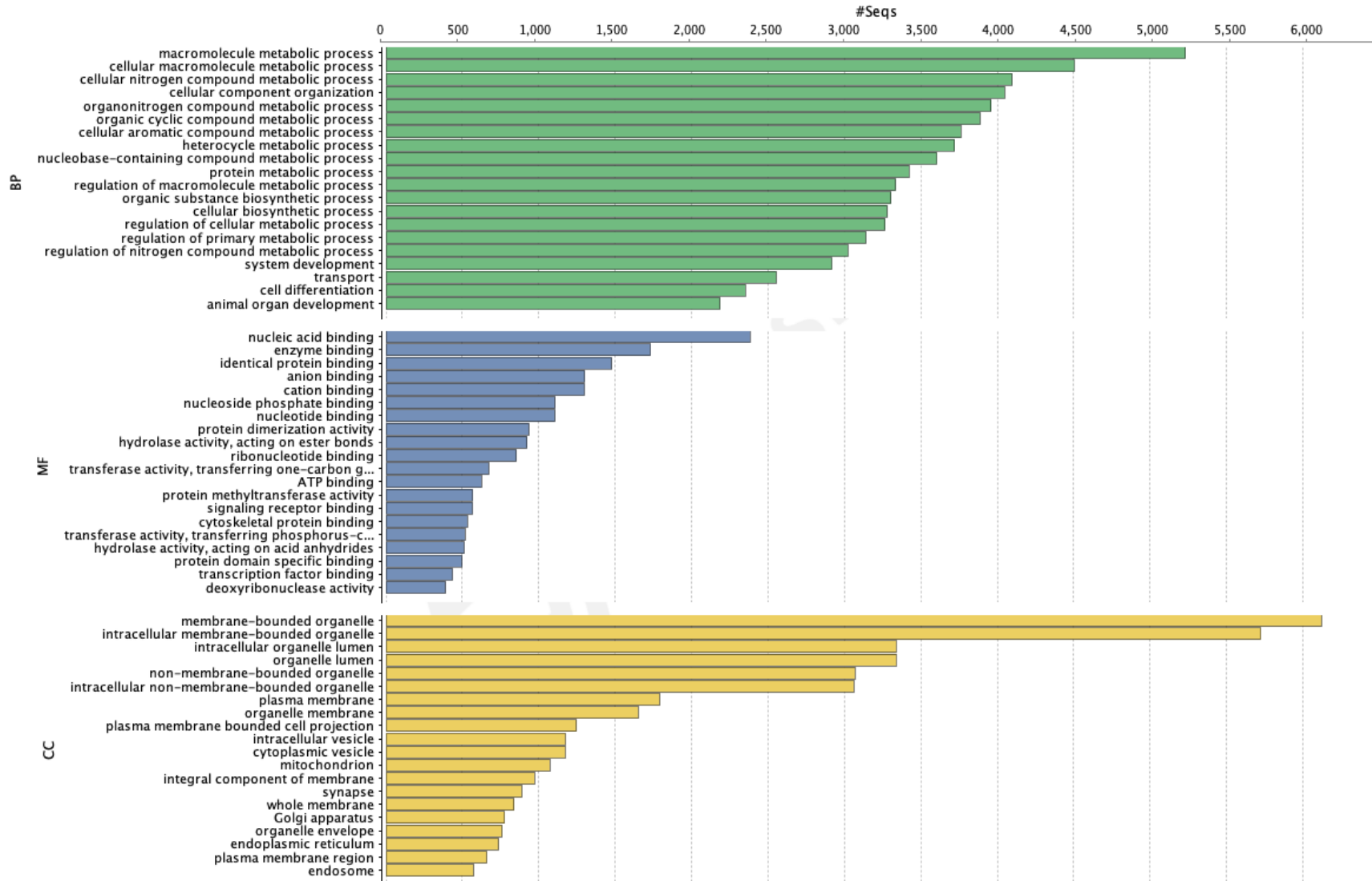
Figure S4. Level four GO terms for the non-redundant merged transcriptome.
