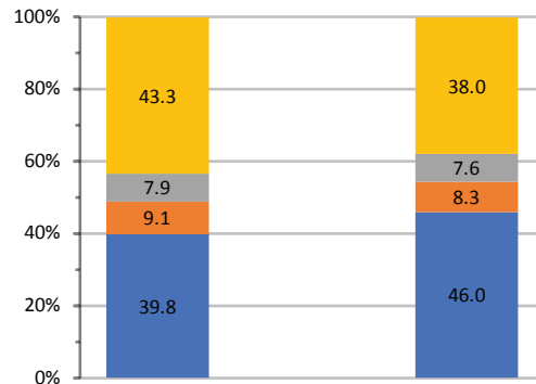
C. goreau (C1)
