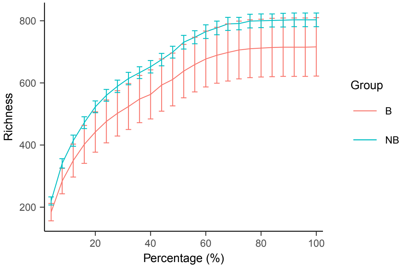
Fig. S1. Alpha diversity rarefaction plots of each group. B, breeding season; NB, non-breeding season.
