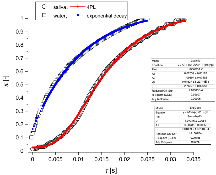
Fitting of the experimental curves \kappa(\tau) for II.A and II.B visualizations.
