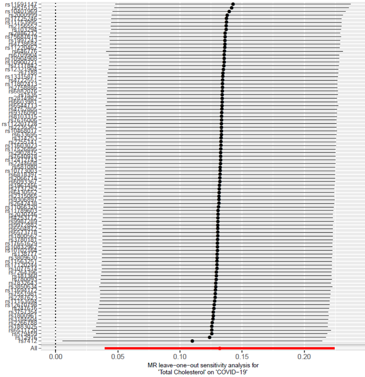
Figure S2 Leave-one-out results for TC to COVID-19.
