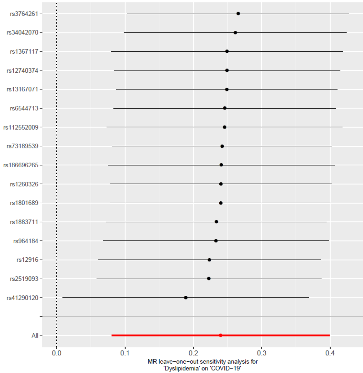
Figure S1 Leave-one-out results for dyslipidemia to COVID-19.
