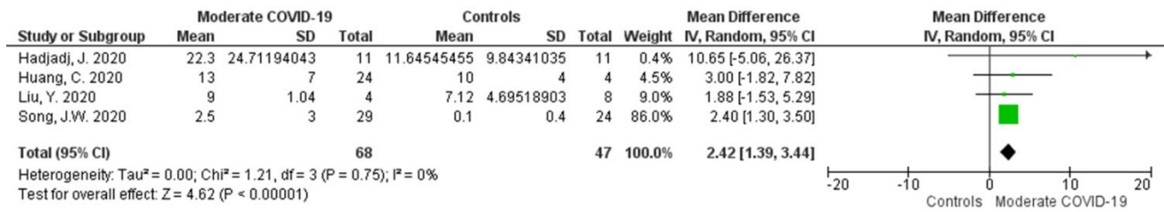
Supplementary Figure 2. Forrest plot for serum IL-17A in COVID-19 patients with moderate disease compared to controls, excluding study with imputed standard deviation.
