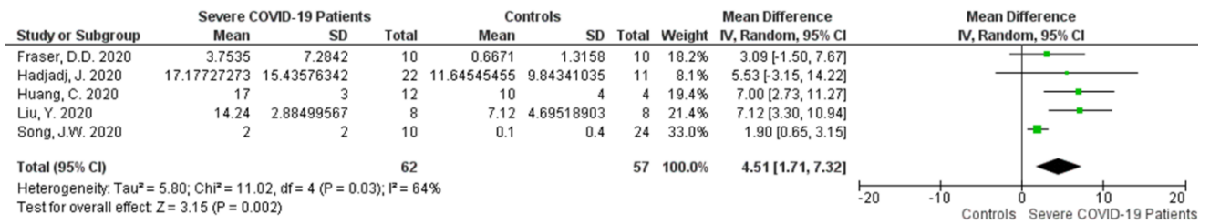
Supplementary Figure 3. Forrest plot for serum IL-17A in COVID-19 patients with severe disease compared to controls, excluding study with imputed standard deviation.
