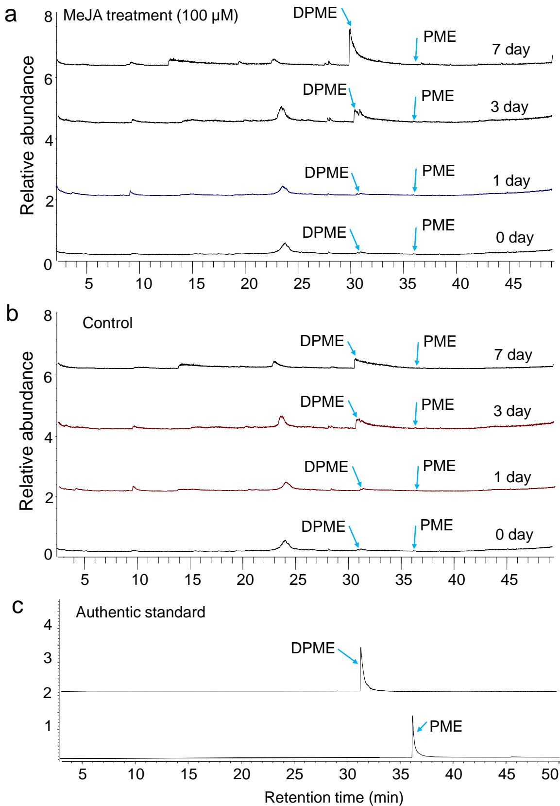
Supplemental Figure S1. GC chromatogram of cell extracts after zero, one, three, and seven days of cell suspension culture treated with (A) or without 100 mg/L MeJA (B). (C) GC chromatogram of standard DPME and PME compounds.
