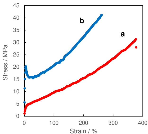
Figure 4. Stress–strain curves of the solvent-cast P(88 mol% 2HB- b -3HB) film above [32°C a , red] and/or below [25°C b , blue] its glass transition temperature.
