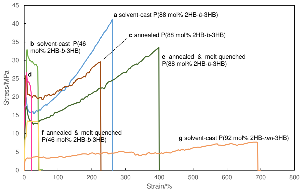
Figure 3. Stress–strain curves of the P(2HB- b -3HB) and P(2HB- ran -3HB) films. a solvent-cast P(88 mol% 2HB- b -3HB) (blue), b solvent-cast P(46 mol% 2HB- b -3HB) (light green), c annealed P(88 mol% 2HB- b -3HB) (brown), d annealed P(46 mol% 2HB- b -3HB) (pink), e P(88 mol% 2HB- b -3HB) annealed and melt-quenched (dark green), f P(46 mol% 2HB- b -3HB) annealed and melt-quenched (yellow), g solvent-cast P(92 mol% 2HB- ran -3HB) (orange). All tests were performed at 25°C.
