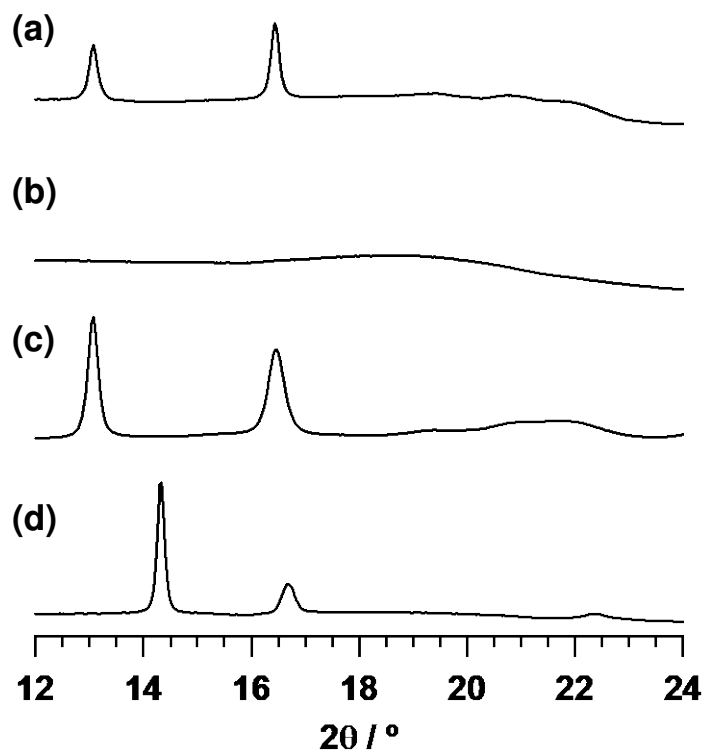
Figure 1. WAXD profiles of a P(88 mol% 2HB- b -3HB), b P(2HB- ran -3HB), c P(3HB), and d P(2HB) films.
