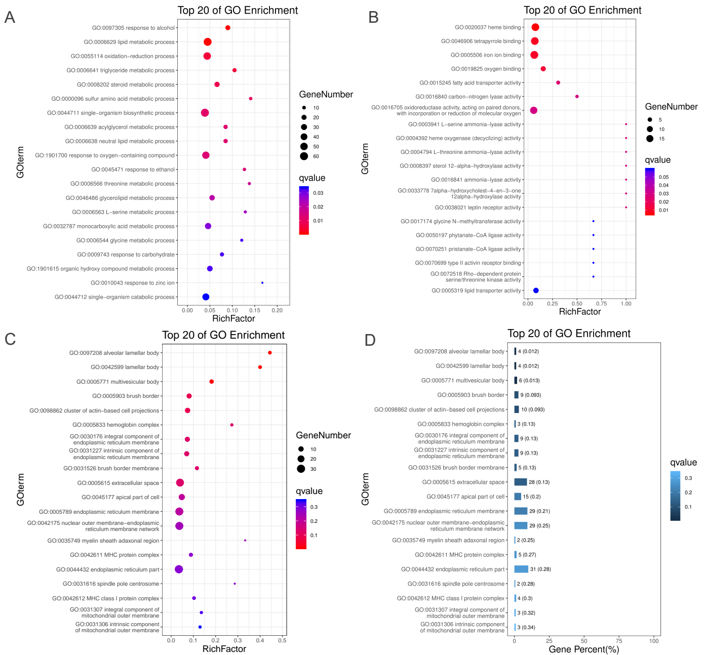
Fig S4. GO enrichment results of all DEGs. (A) Top 20 of GO enrichment on Biological process; (B) Top 20 of GO enrichment on Molecular Function; (C) Top 20 of GO enrichment on Cellular component. (D) Top 20 of GO enrichment on Cellular component by bar plot.
