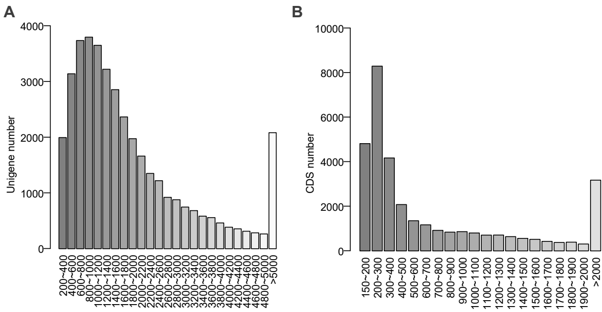
Fig S1. Sequence length distributions of unigene and CDS. (A) Unigene length distribution. The minimum unigene length > 200 nt, x-axis represents fixed length, and y-axis for the corresponding unigene counts. (B) CDS length distribution. The minimum CDS length is 150 nt. X-axis represents fixed length, and y-axis for the corresponding CDS counts.
