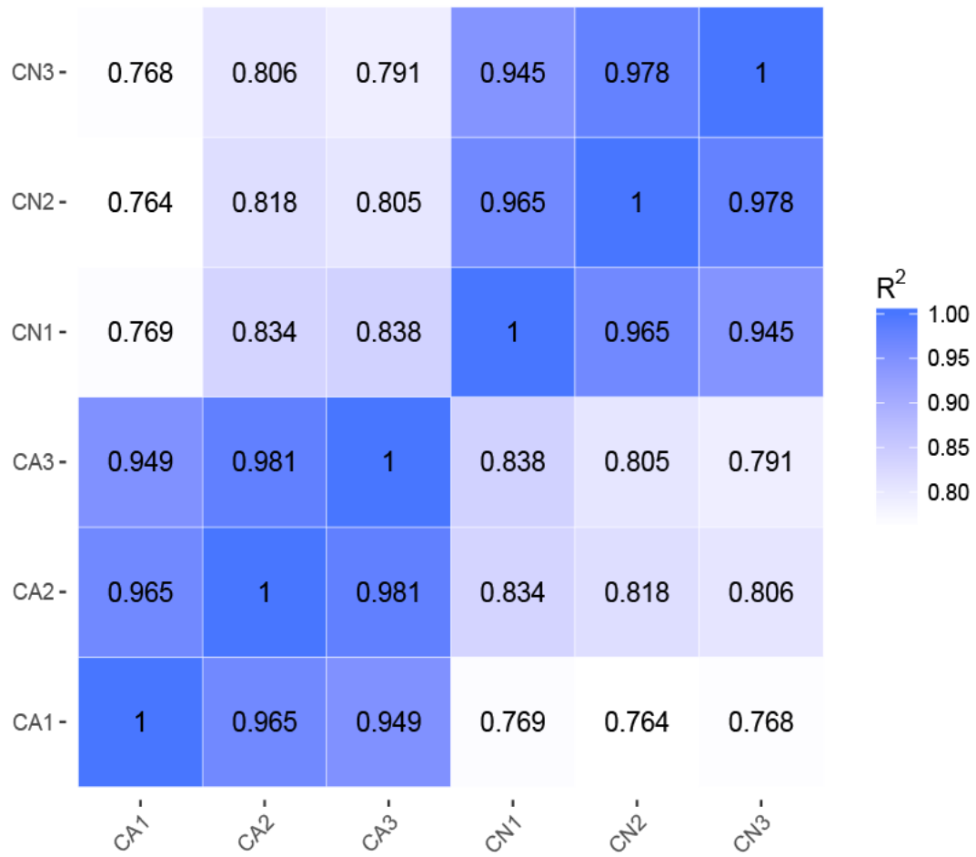
Figure S1 The pearson correlation between samples.
