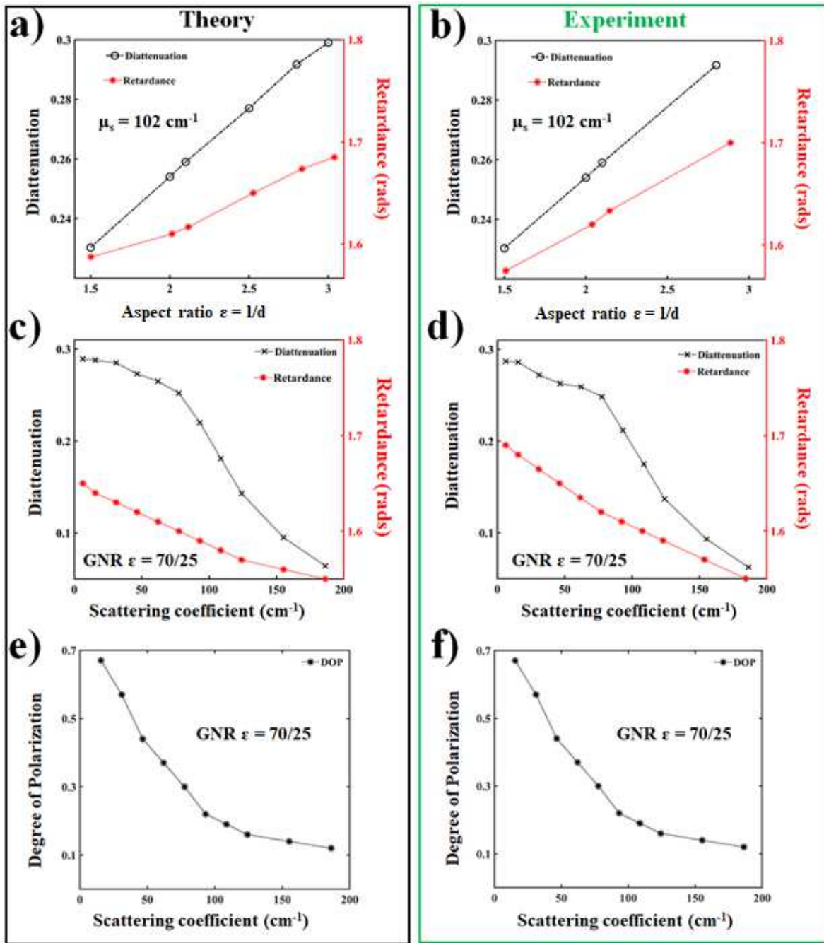
Figure 3. Polarization effects in a composite microsphere + GNRs phantom system. Mueller matrix simulated (a) and experimentally obtained (b) variation of the diattenuation (left axis, black symbols) and retardance (right axis, red symbols) with GNR's aspect ratio \epsilon for a fixed scattering coefficient of the composite system ( \mu_s = 102 \text{ cm}^{-1} due to microspheres plus \mu_s = 16 \text{ cm}^{-1} due to GNRs). Increasing diattenuation and retardance with aspect ratio suggests size-dependent increase of the optically anisotropic nature of GNRs. Simulated (c) and experimental (d) variation of diattenuation and retardance with GNRs concentration in a turbid phantom of fixed microsphere scattering properties (diameter = 0.42 \mu\text{m} , \mu_s = 102 \text{ cm}^{-1} ). The geometrical parameters of GNRs were length l = 70 \text{ nm} , diameter d = 25 \text{ nm} (aspect ratio \epsilon = 2.8 ). Both D and R exhibit significantly higher values (better contrast) at lower nanorod concentrations ( \mu_s = 16 \text{ cm}^{-1} ), implying strong orthogonal dipolar plasmon polarizabilities even for 3D random orientations of GNRs (for details, see text). The corresponding simulated (e) and experimental (f) dependence of the surviving degree of polarization on the GNR concentration.
