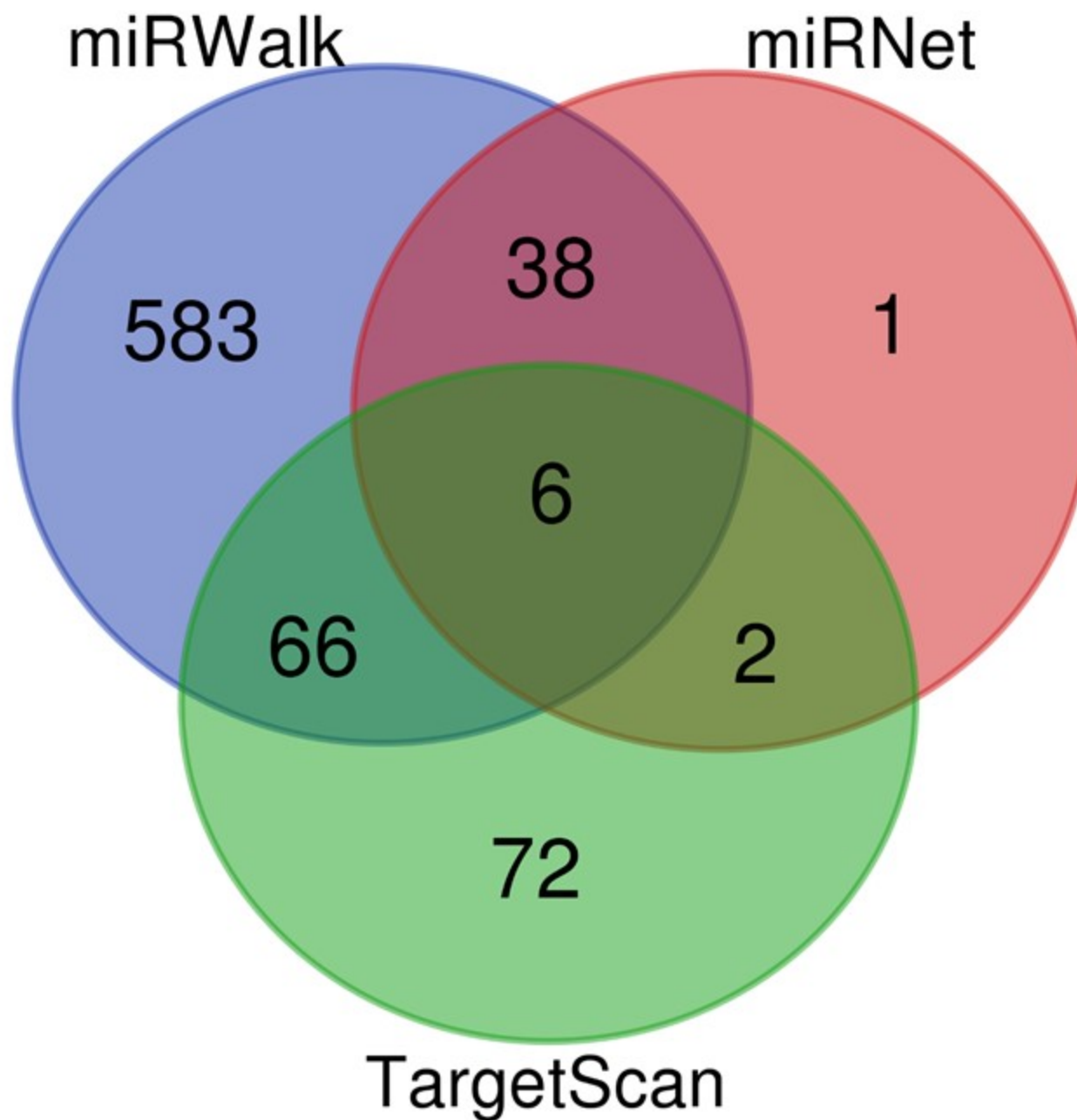
Supplementary Figure 2. Venn diagram involving the three miRNAs prediction software; miRWalk, miRNet, and TargetScan. The blue circle represents the number of miRNA predicted by miRWalk (693), pink miRNet (47), and green Target Scan (146). The center region represents the six miRNAs used for further analysis in this study.
