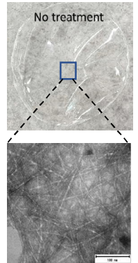
TO-CNF film
