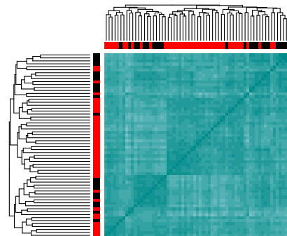
Colon – RR, J=2
