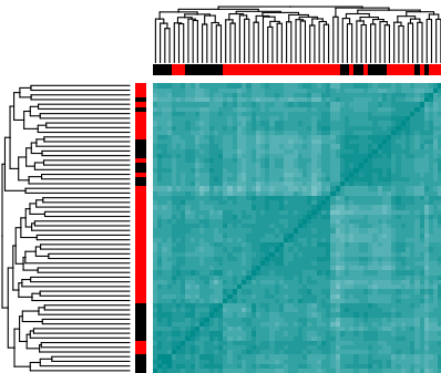
Colon – Jaccard, J=2
