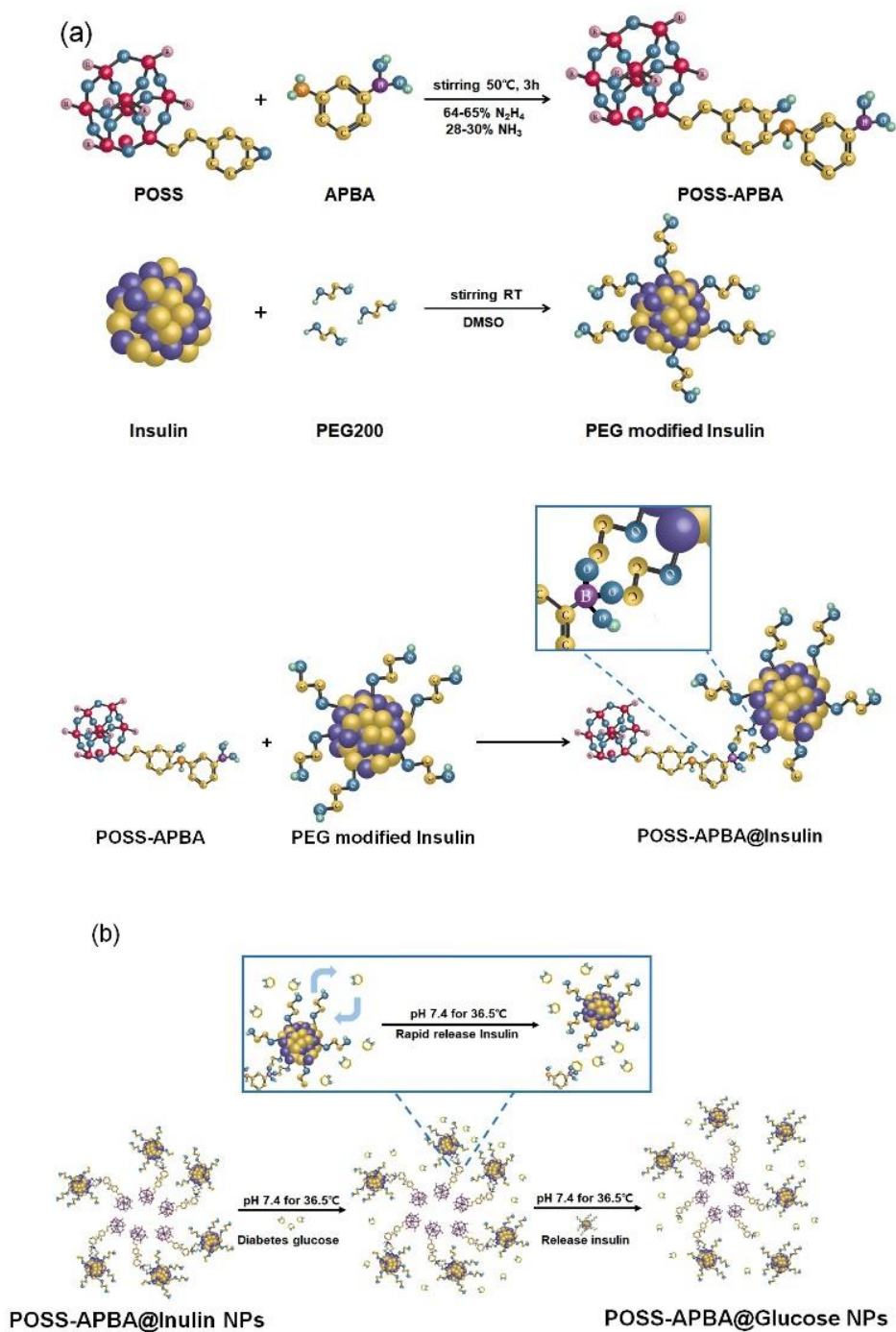
Scheme 1. (a) Synthesis design of POSS-APBA, PEG modified Insulin and POSS-APBA@Insulin (b) Insulin releasing mechanism of glucose specific response by POSS-APBA@Insulin at pH 7.4 at 36.5°C.
