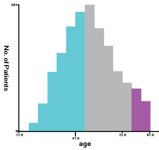
Fig.S1 The cut-off values of age were found by x-tile software .
