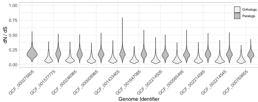
S2 Fig. Full results on dN/dS ratios obtained with proteins no more that 70% identical. The results still show orthologs to have lower dN/dS values than paralogs.
