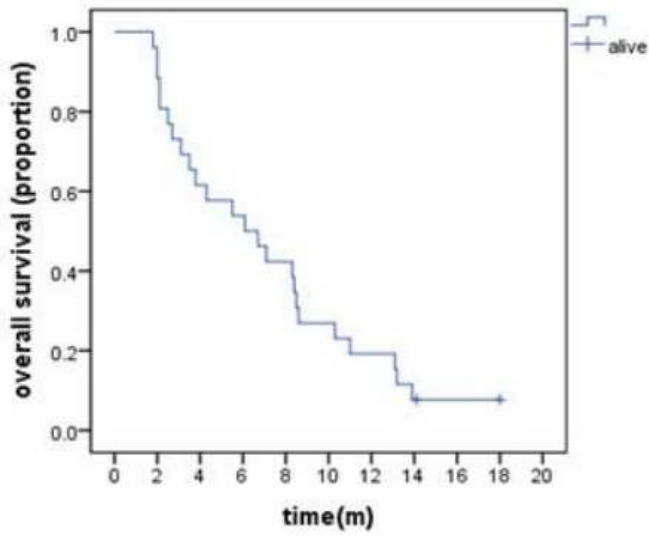
Figure 1A : Survival functions
