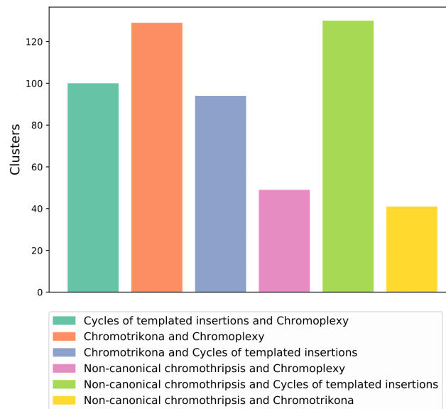
Figure S3: Common clusters between every pair of triangle types.
