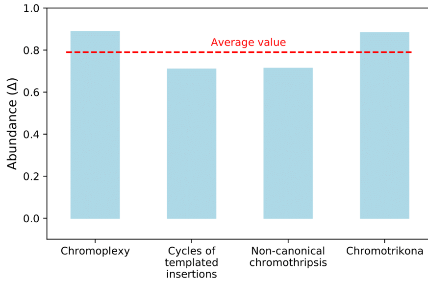
Figure S2: Abundance values for different triangle categories.
