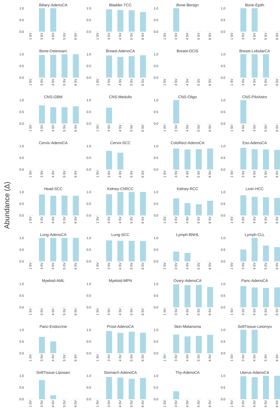
Figure S1: Abundance values of the evaluated cycles for the 36 cancer types. Cycles with an Abundance = 0 do not have any pattern both in the simulation and in the original dataset.
