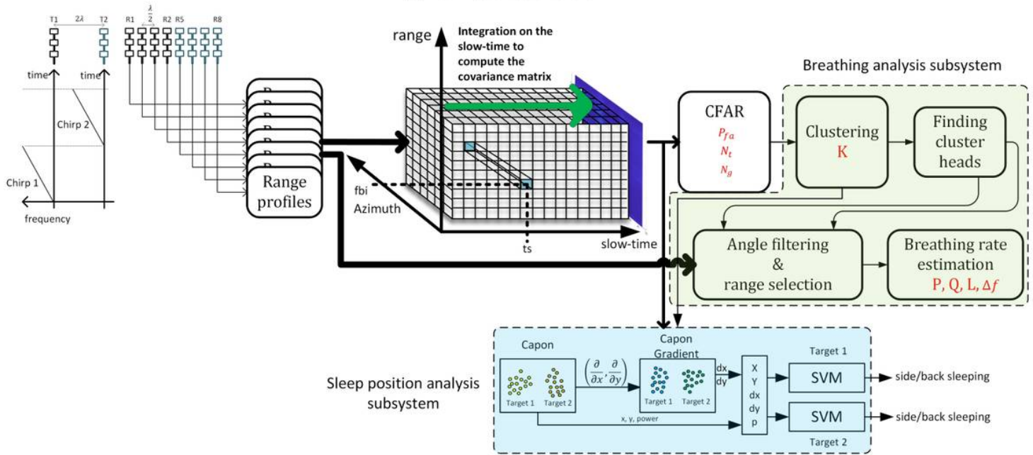
(b) Signal processing flow and the parameters
