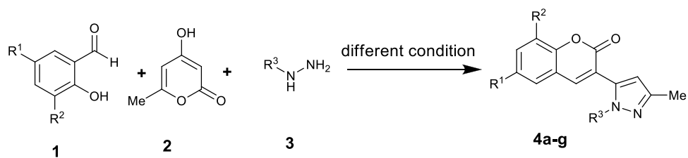
Scheme 1: Different conditions of the synthesis of chromenone-pyrazole derivative
