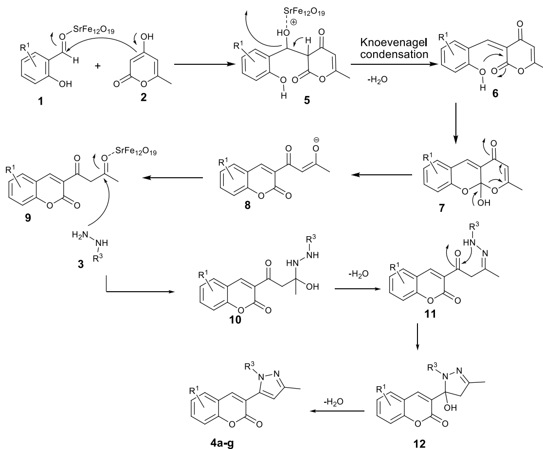
Scheme 2: The proposed mechanism for the synthesis of chromenone-pyrazole compounds ( 4a-4g )
