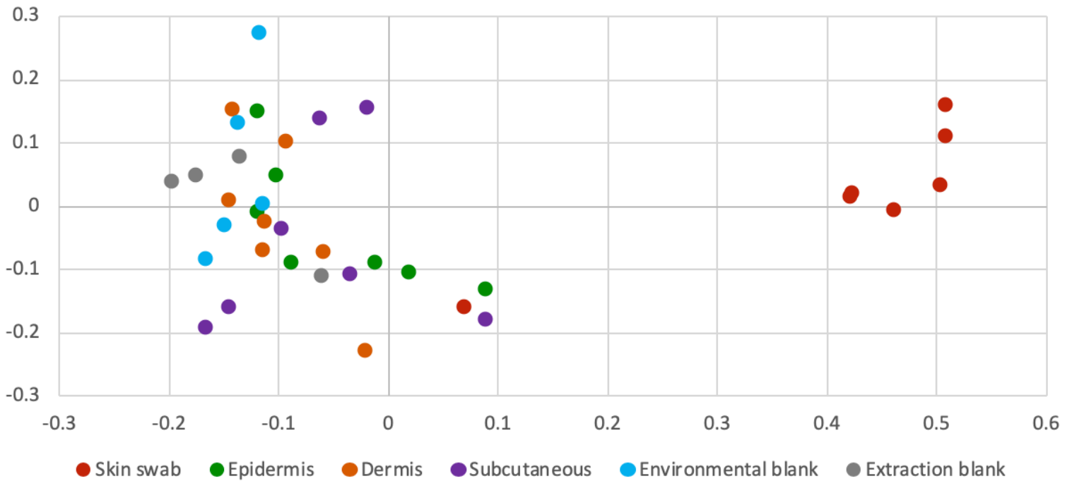
PCoA Unweighted UniFrac
