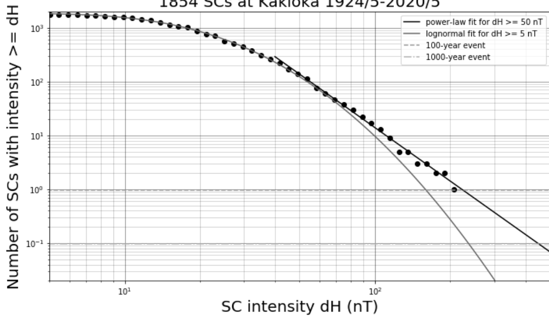
1854 SCs at Kakioka 1924/5-2020/5
