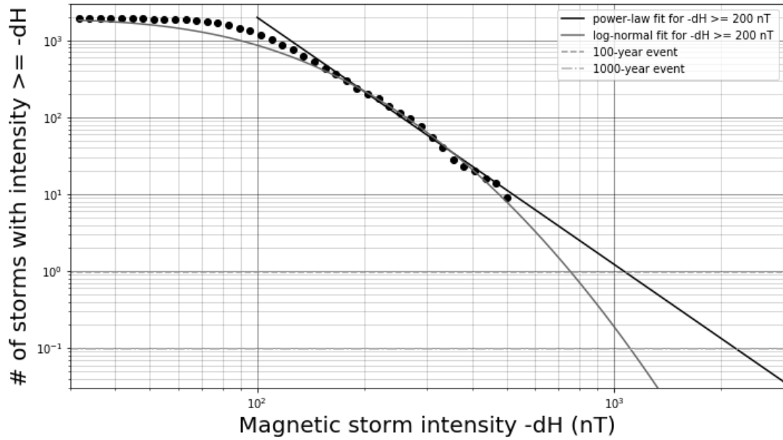
1921 Storms at Kakioka 1924/5-2020/5
