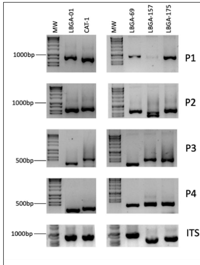
Fig S1 – Molecular characterization of the thermotolerant strains. Four polymorphic regions of SPA2 (P1), PYR3 (P2), MNN4 (P3) and EPL1 (P4), genes were amplified according described by Carvalho Netto [10]. The ITS amplification were done using primers described by Uranska et al. [11].
