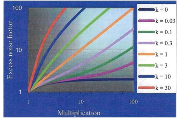
Figure 2: McIntyre's curves
