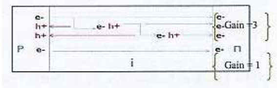
Figure 1: Avalanche multiplication
