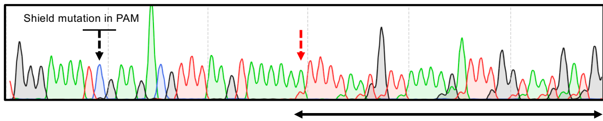
Figure S2. Sequence analysis of pfap2-g-ko parasites. The genomic DNA was purified from the parasite harvested before the limiting dilution and then sequenced. The PAM sequence, TGG, was mutated to the TCG almost completely, as indicated by the black arrow. While one adenine insertion was detected as indicated by the red arrow (refer to Fig. 3C), the minor histograms were also detected. Those minor histograms were frequently detected in downstream of the site where the adenine was inserted. These were derived from the wild-type sequences.
