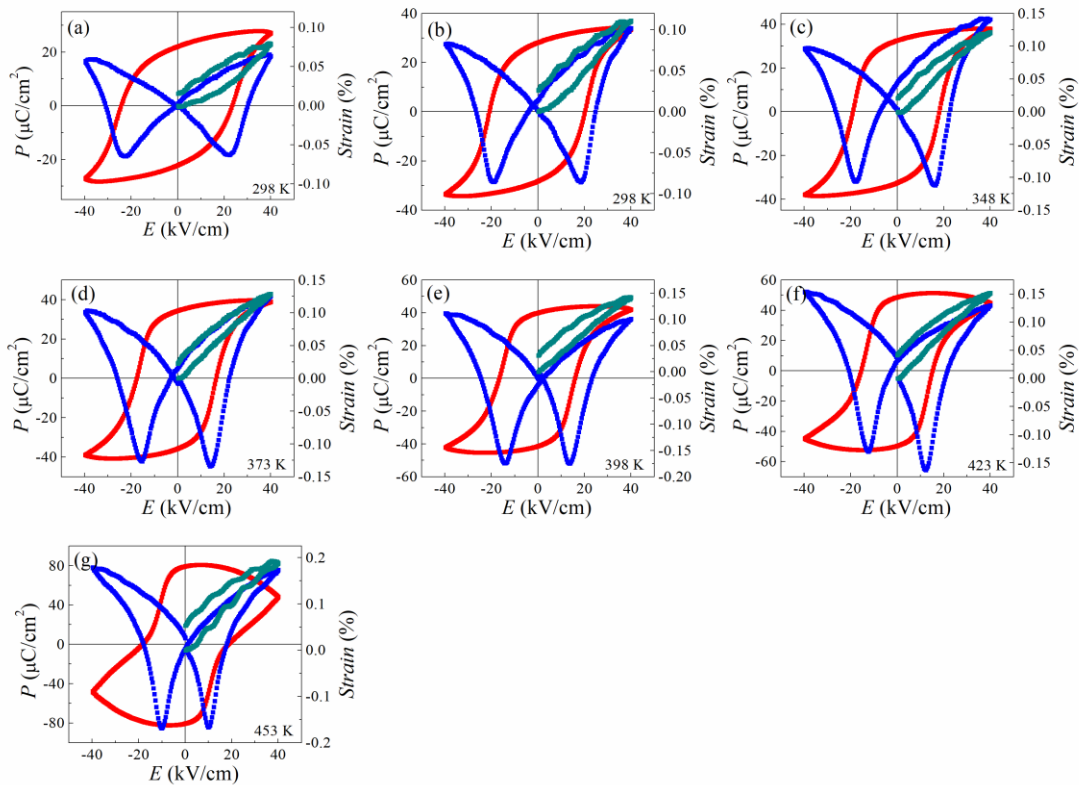
Fig. S1 Polarisation, bipolar and unipolar responses at various temperatures
