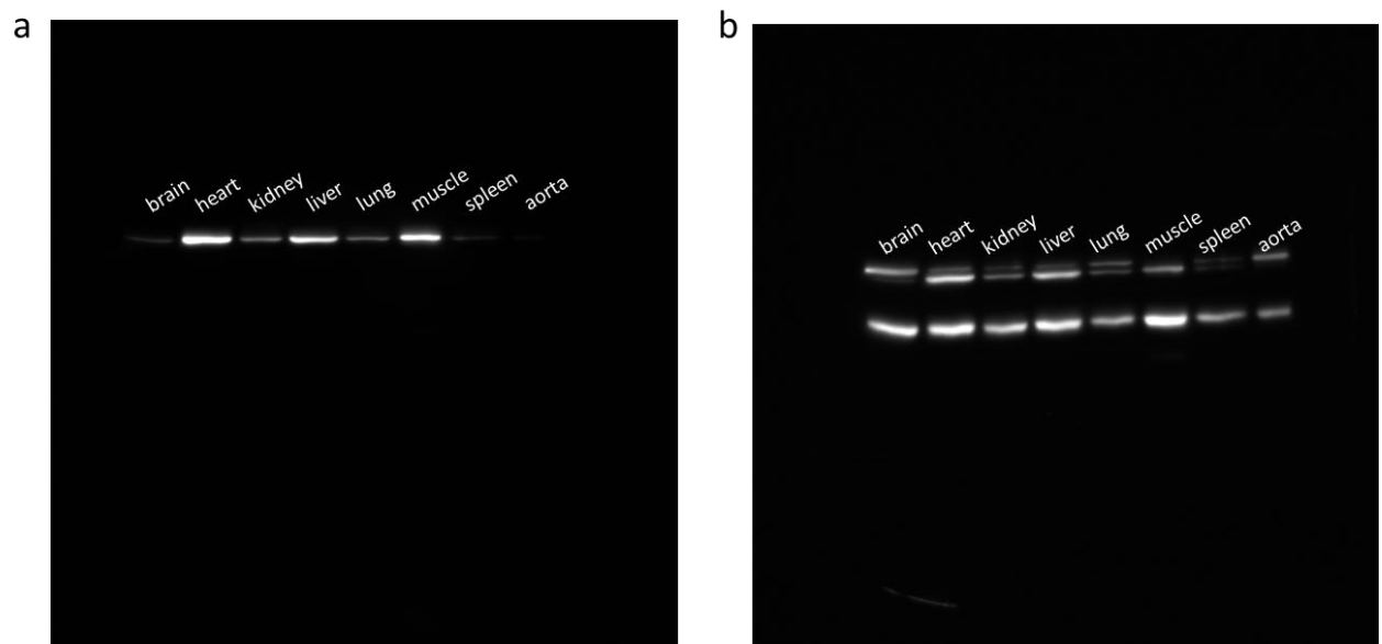
Supplementary Figure 1. Distribution of AGXT2 transgene in different tissues of TG mice, detected by Western blotting (unprocessed data). (a) AGXT2-FLAG, (b) GAPDH.
