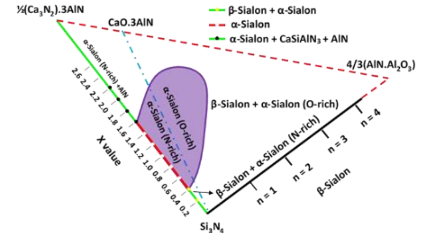
Phase Stability Along N'Rich Line (1500°C)
