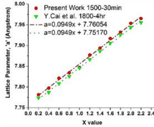
Increase in lattice parameters with Ca in \alpha Sialon Unit Cell
