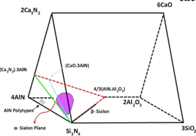
Janecke Prism with Ca- \alpha Sialon Plane (1800°C)
