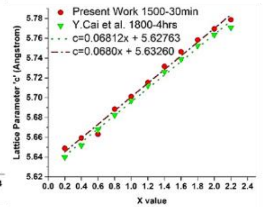
Increase in lattice parameters with Ca in \alpha Sialon Unit Cell
