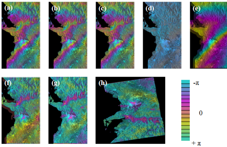
45 Figure 4. Interferograms produced during the procedure of correction of ionospheric 46 disturbances for the pair of images April 26 and June 21, 2016 of P131-F640. (a) 47 Original differential interferogram in radar coordinate. (b) Interferogram for higher 48 band. (c) Interferogram for lower band. (d) Double differenced interferogram; i.e. 49 difference between higher and lower band interferograms. (e) Estimated ionospheric 50 components. (f) Non-dispersive components in original interferogram; i.e. subtracted 51 phase of ionospheric components from original one. (g) Flattened and filtered non- 52 dispersive components of interferogram. (h) Geocoded flattened and filtered non- 53 dispersive components of interferogram.
