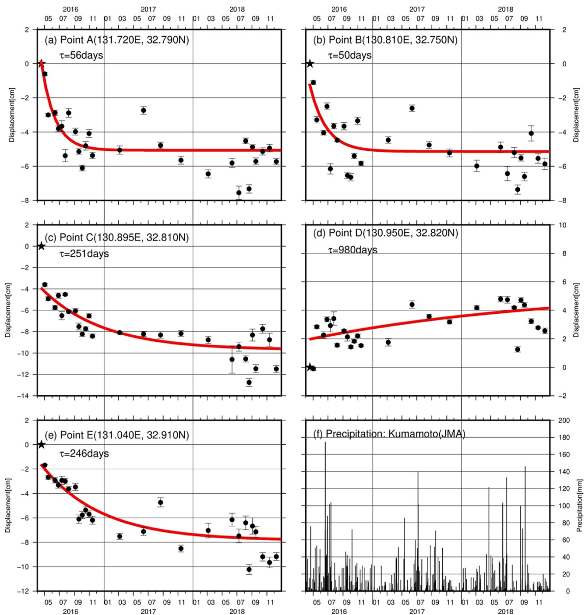
126 Figure 12. (a) - (e) Time series plot of LOS changes at 5 spots in the descending 127 interferogram in Figure 9b. Average of LOS change in an area of 0.05^\circ \times 0.05^\circ centered 128 at the point shown in each diagram. Error bar indicates 1-sigma. Red line is the best fit 129 exponential decaying curve, whose characteristic time is shown in the diagram. (f) 130 Daily precipitation in mm at JMA Kumamoto station in the Kumamoto City [JMA, 131 2020].
