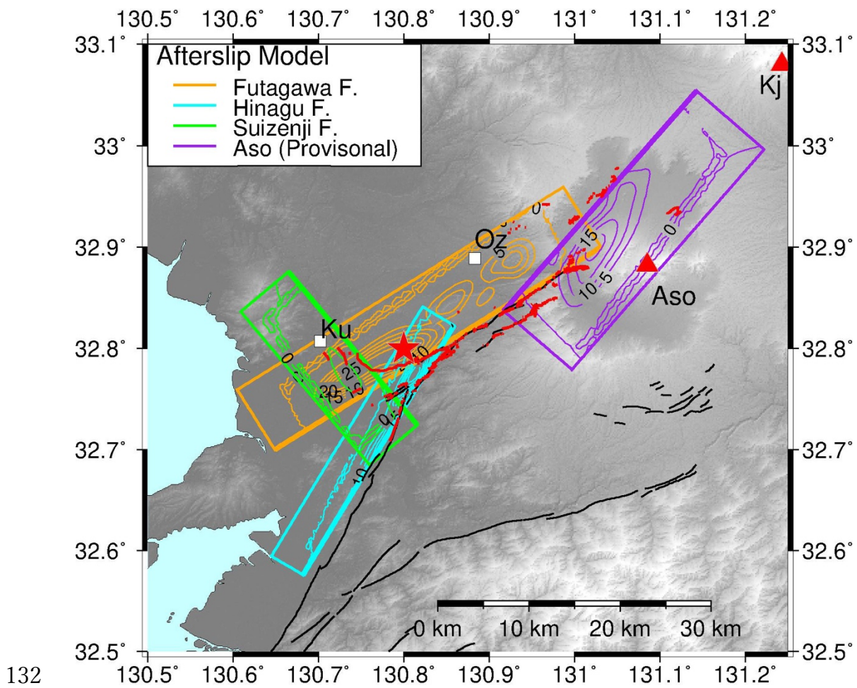
132 Figure 13. Compilation of modeled faults. Orange, blue, green and purple indicate 133 Futagawa, Hinagu and Suizenji faults and provisional fault in Aso caldera, respectively. 134 Unit of contours of slip is cm/yr.
