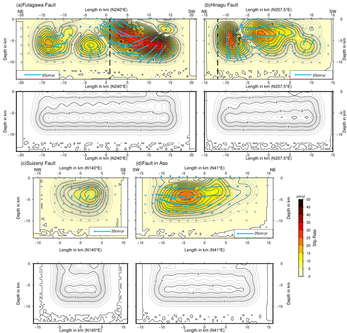
138 Figure. 14. Distribution of estimated slip (top) and errors (bottom) projected onto 139 vertical plane along strike. Blue arrows are slips of the hanging-wall side relative to the 140 foot wall side. Unit of contours are cm/yr. (a) Futagawa fault. Dip angle is 74°. (b) 141 Hinagu fault. Dip angle is 61°. Vertical dashed lines in these figures indicate crossing 142 point of two faults. (c) Suizenji fault. Dip angle is 64°. (d) provisional fault in Aso 143 caldera. Dip angle is 55°.
