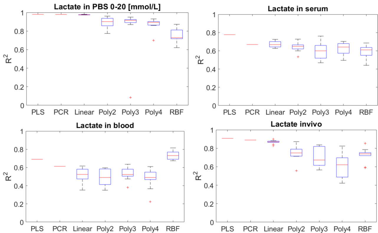
Figure 2 The comparison of the performance of linear and nonlinear models in increasingly more scattering matrices. The boxplots summarise the results pertaining to ten runs of cross-validation for each model. After each run, an estimate of the coefficient of determination, R^2 , is obtained.
