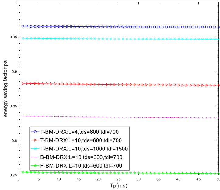
FIGURE 4. Relationship between sleep-ready timer and energy saving.
