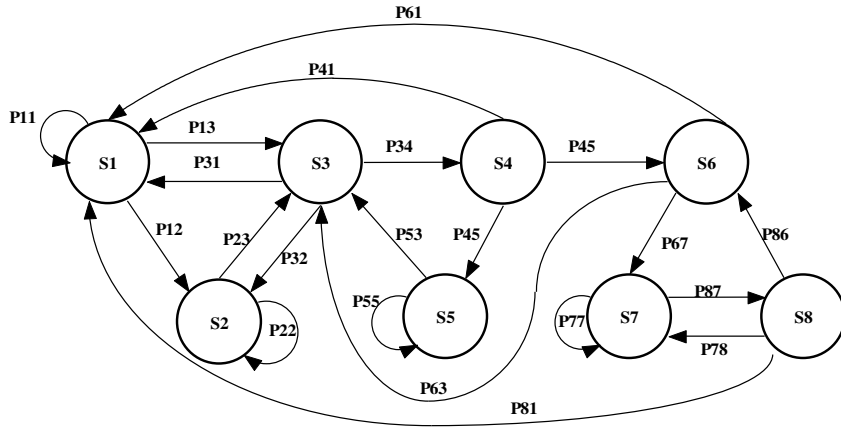
FIGURE 3. Markov chain of BM-DRX.
