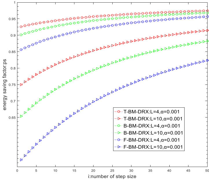
FIGURE 6. Effects of t_{ds} and t_{dl} on energy saving.
