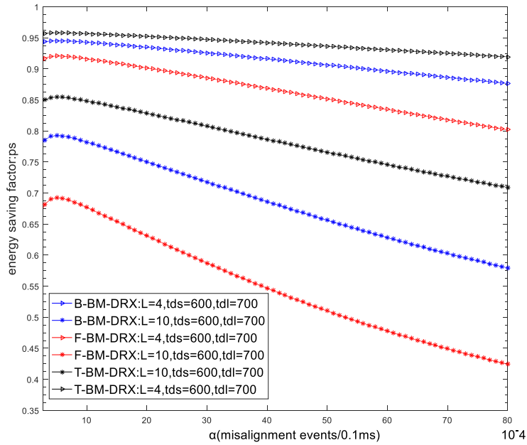
FIGURE 5. Effects of beam misalignment rate on energy saving.
