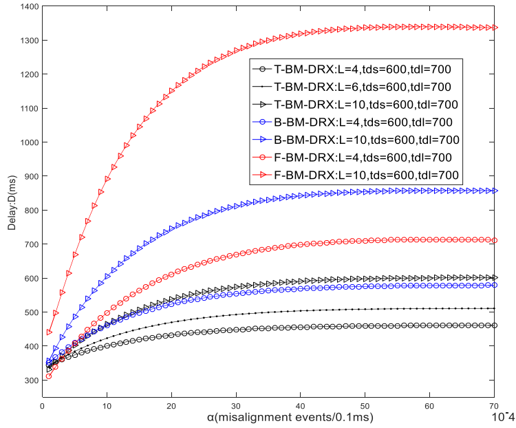
FIGURE 7. Effects of misalignment rate on delay.
