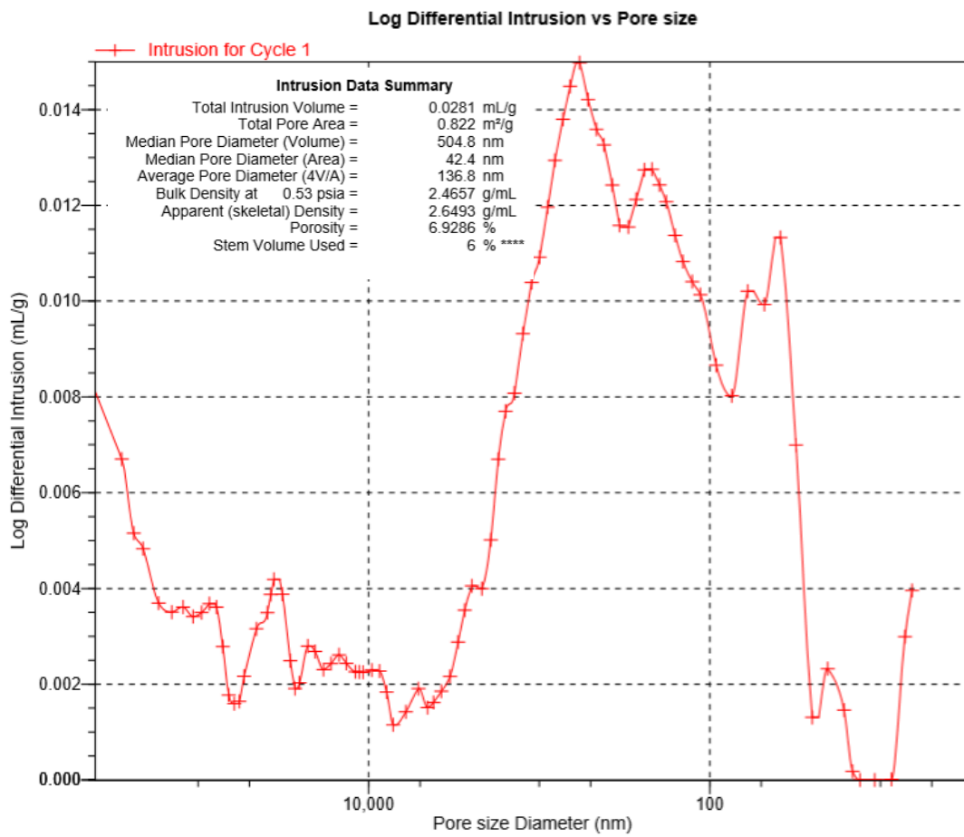
Figure 2. Pore structure analysis using MIP method (MICROMERITICS)
