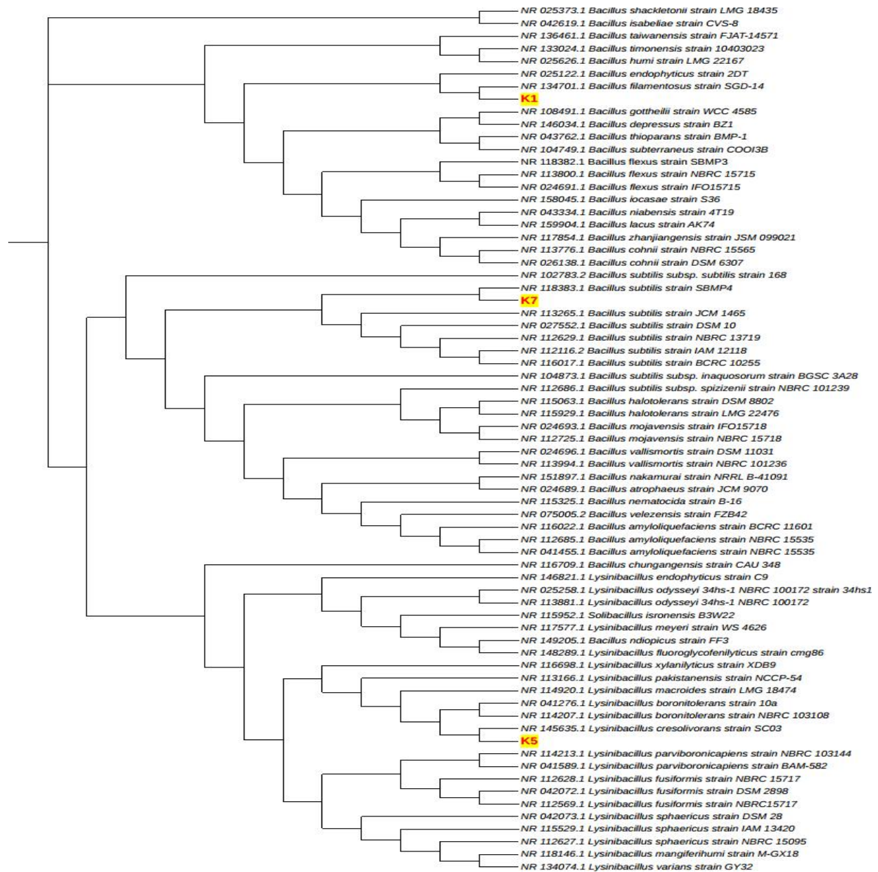
Figure S1. Maximum likelihood phylogenetic tree of the bacterial isolates K1, K5 and K7.
