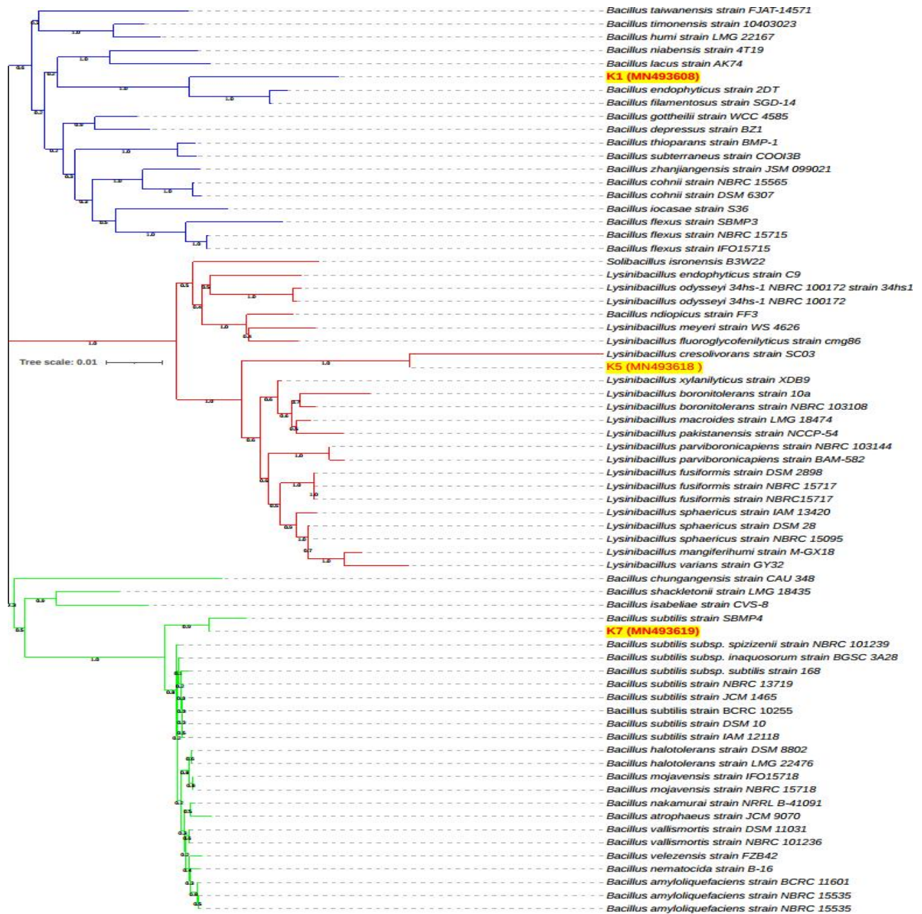
Figure S2. Neighborhood phylogenetic tree of the selected bacterial isolates K1, K5 and K7.
