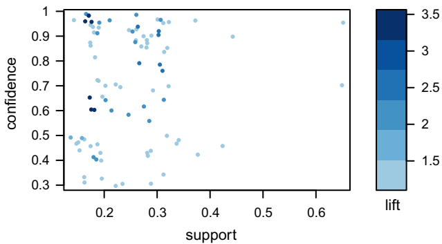
Scatter plot for 88 rules
