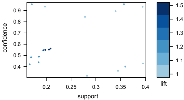
Scatter plot for 18 rules
