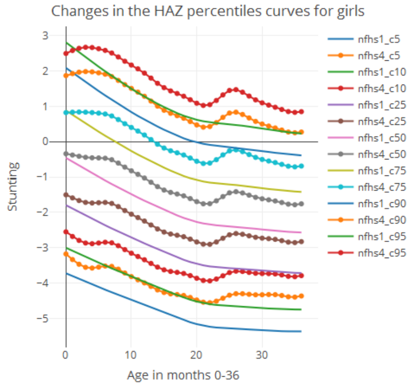
Figure 1: LMS curves for child aged 0-36 months in NFHS 1 (1992) and NFHS 4 (2016)
