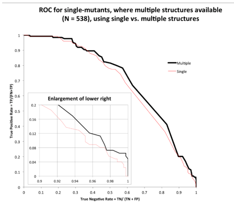
Figure 4. Receiver Operating Characteristic, comparing homologyScanner vs. calculation on single structures.
