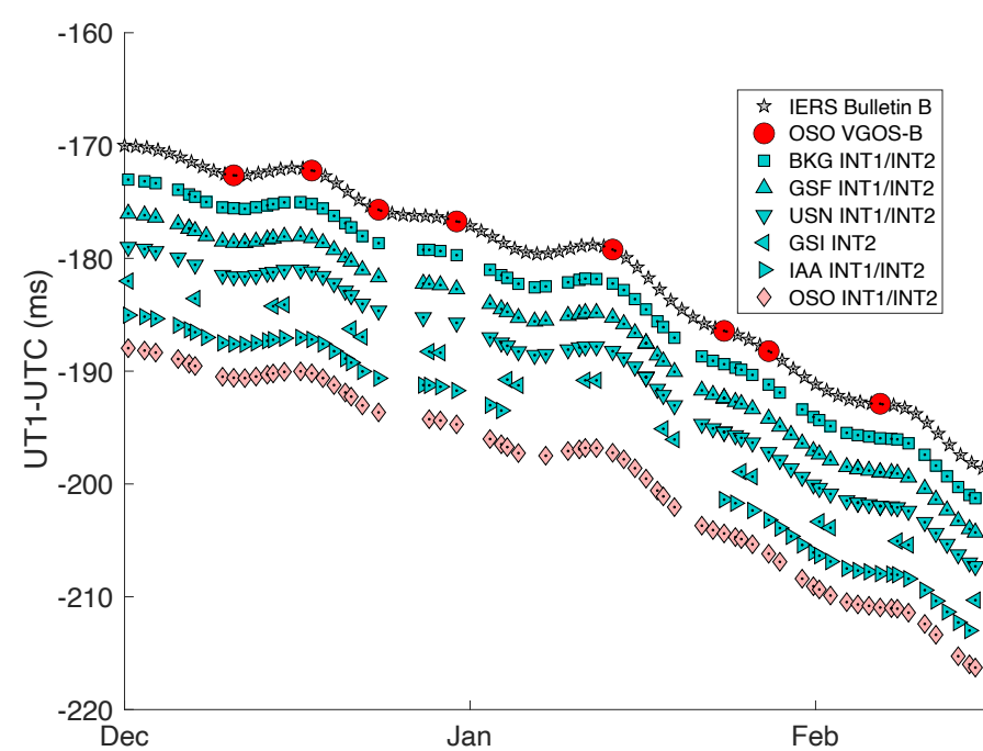
UT1-UTC from legacy S/X and VGOS-B
