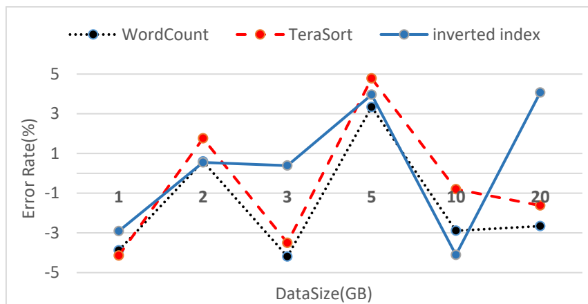
Fig. 9- The percentage error rate on 13 nodes
