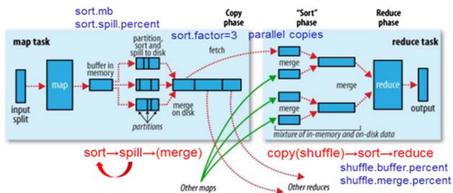
Fig. 2- Parameters that affect Hadoop pipeline [1, 11]
