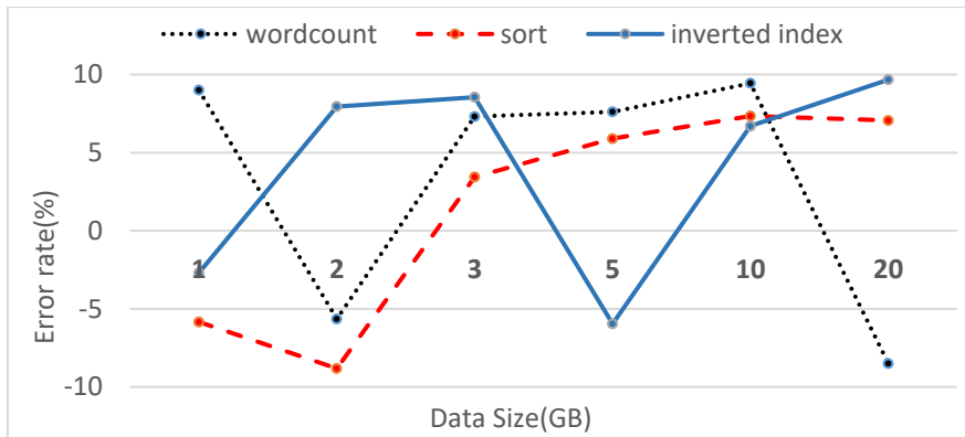
Fig. 6 - The percentage error rate on 3 nodes
