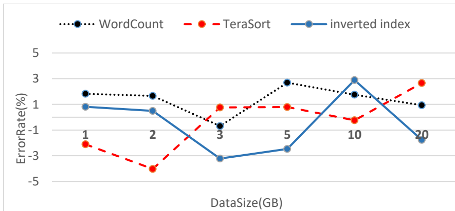
Fig. 12 - The percentage error rate on 3 nodes
