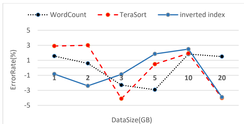
Fig. 10- The percentage error rate on 10 nodes
