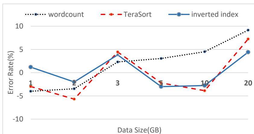
Fig. 4 - The percentage error rate on 10 nodes
