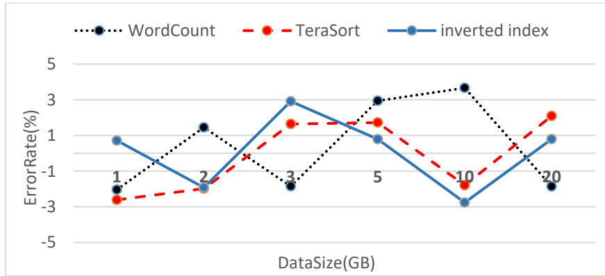
Fig. 11- The percentage error rate on 5 nodes
