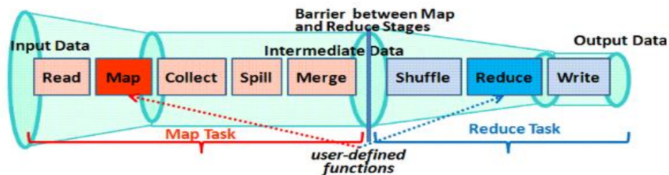
Fig. 1 - MapReduce processing pipeline [2]
