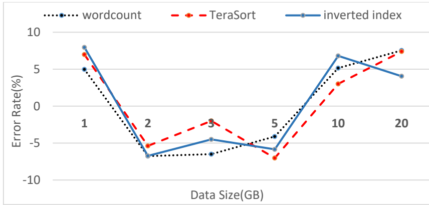
Fig. 5 - The percentage error rate on 5 nodes
