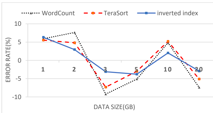
Fig. 3 - The percentage error rate on 13 nodes
