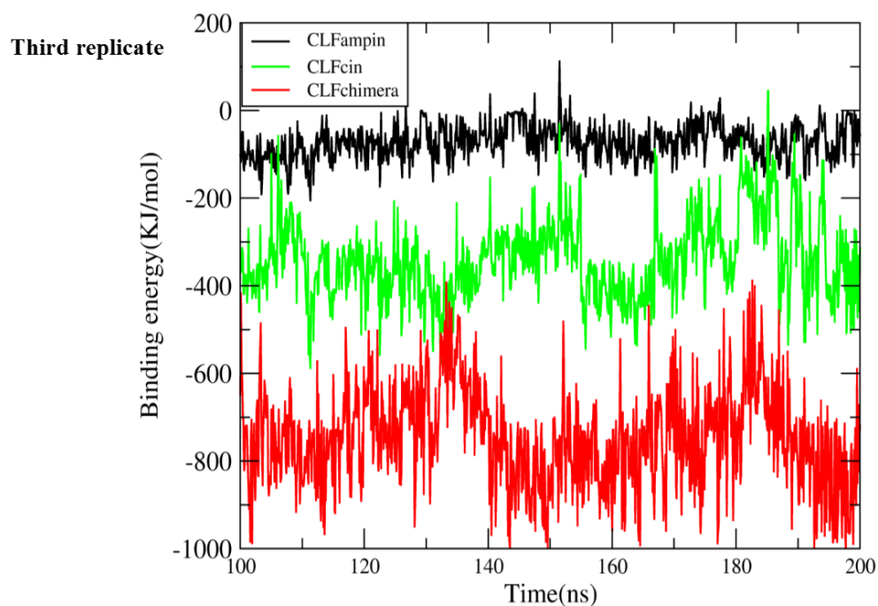
Figure S8. Second and Third replicates: Estimated binding free energy for the peptide-DNA systems. Calculated with the MM/PBSA method on the 100-200 ns period of one of the simulation replicates.
