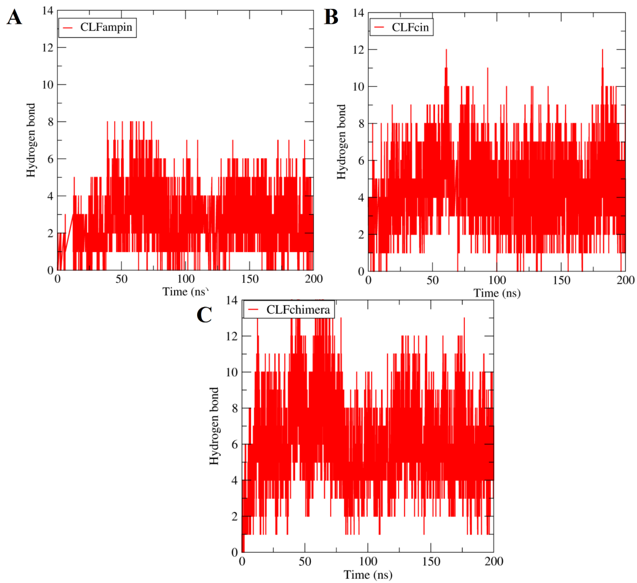
Figure S6. Third replicate: Number of hydrogen bonds with DNA as function of simulation time (200 ns). (A) CLFampin, (B) CLFcin, (C) CLFchimera
