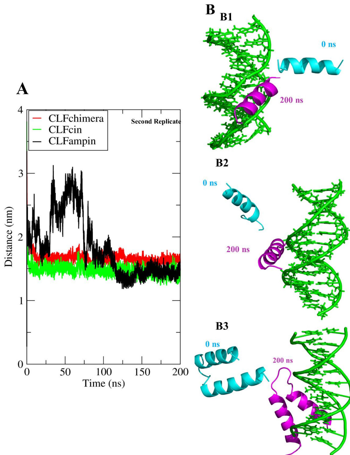
Figure S3. Second replicate: COM distance analysis. (A) COM distances between CLFcin, CLFampin and CLFchimera and DNA along 200 ns. (B) Structures at times t=0 (cyan) and t=200 ns (purple): (B1) CLFcin-DNA, (B2) CLampin-DNA, and (B3) CLFchimera-DNA.
