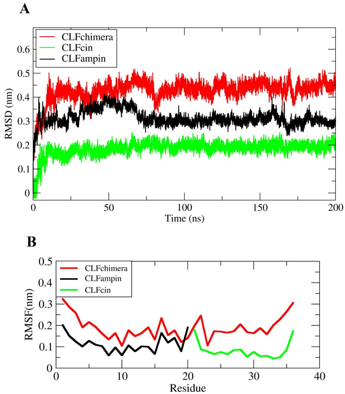
Figure S2. Third replicate: Structural fluctuation analysis. (A) RMSD as function of time; (B) RMSF per residue
