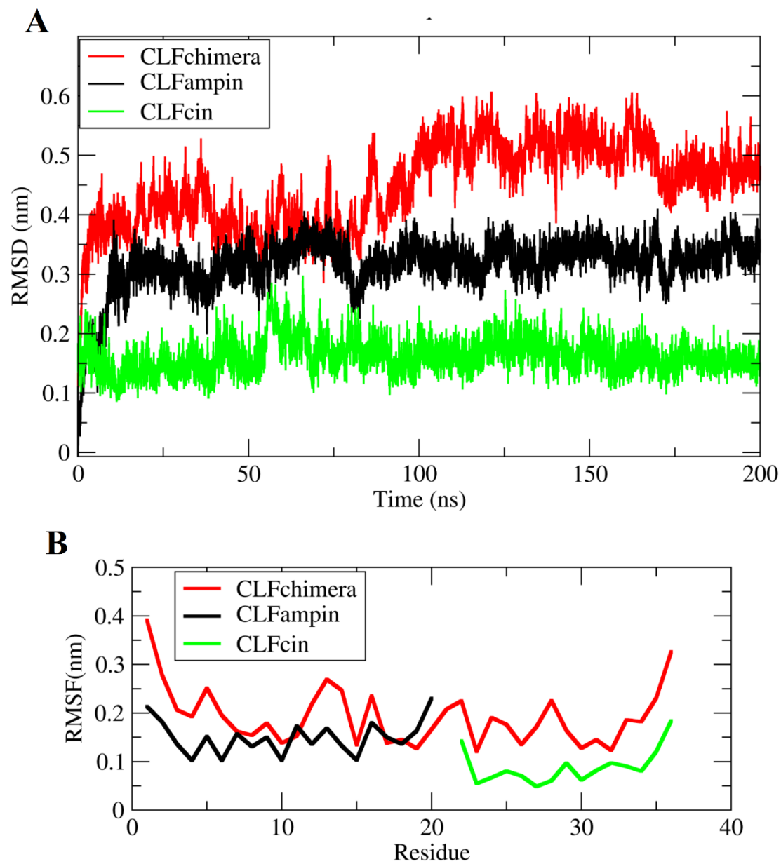
Figure S1. Second replicate: Structural fluctuation analysis. (A) RMSD as function of time; (B) RMSF per residue
