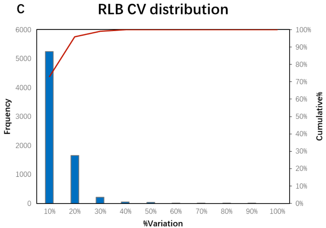
Supplementary Fig. 7 The repeatability of quantification data among three biological replicates of each group (A: DSB; B: ASB; C: RLB) according to their quantitative data. Red line means the cumulative curve.
